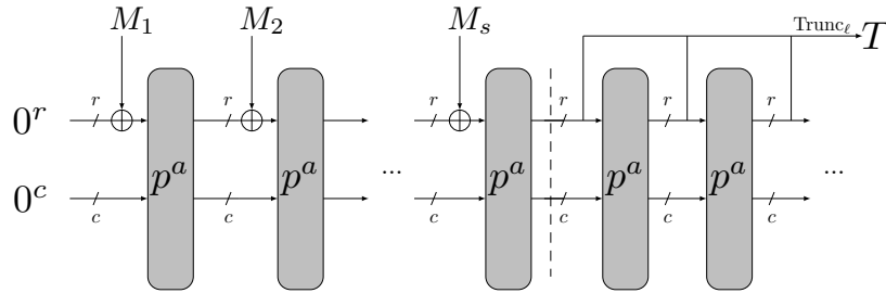
Figure 1: Sponge function
